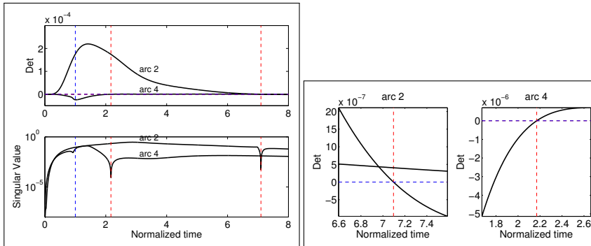
Fig. 5 Fluid case, step 4: second order conditions. Second order necessary condition checked on solution 1/12 with \lambda = 2.0 from Table 3. The rank condition from the algorithm presented in subsection 4.3 from [11] is evaluated along the two singular arcs. See [6] for details on the concept of conjugate times. On the left subplot, for each singular arc, the curve is reparameterized so that the final time corresponds to the abscissa 1 (vertical blue dashed line); the determinant associated with the rank condition is plotted (top subgraph), so there is a conjugate time whenever it vanishes (vertical red dashed lines). One observes that conjugate times on each arc are located after the (normalized to 1) final time, satisfying necessary condition of local optimality of the trajectory. At the bottom, the smallest singular value of the matrix whose rank we test is plotted, extracting only the relevant information to detect the rank drops. On the right subplot is presented a zoom of top-left subgraph near the two conjugate times.
